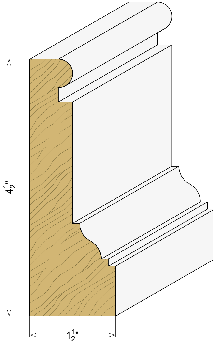
AP 2250 1-1/2" x 4-1/2"
