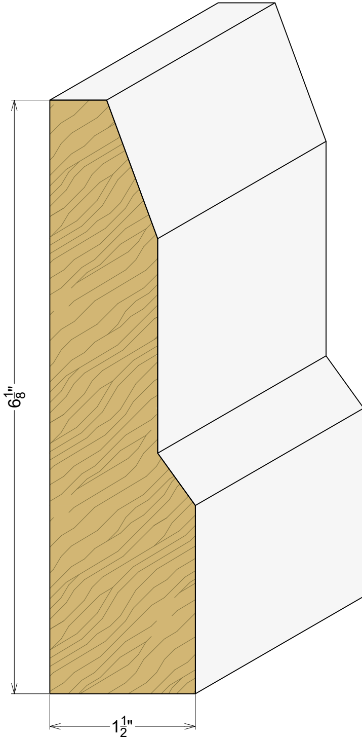
AP 2253 1-1/2" x 6-1/8" Plinth Block
