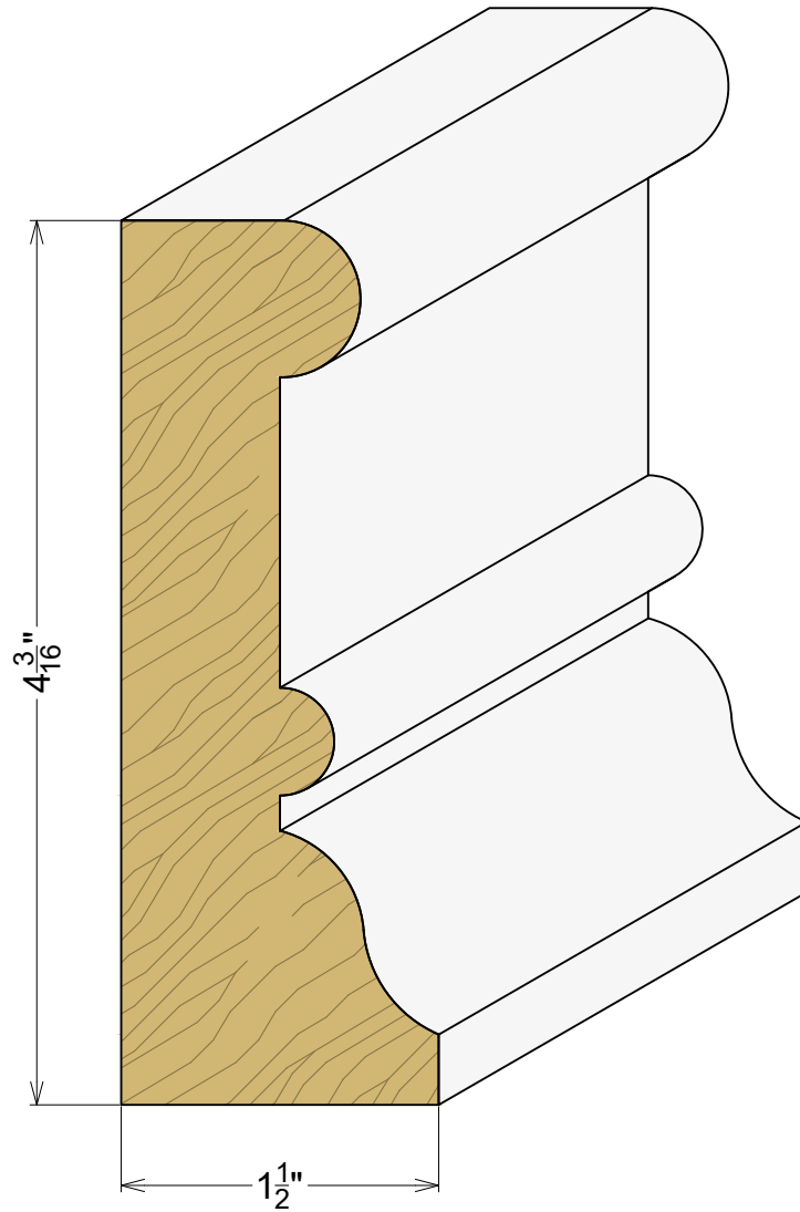
AP 2254 1-1/2" x 4-3/16"
