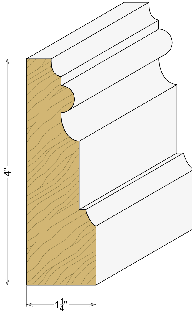
AP 2257 1-1/4" x 4"
