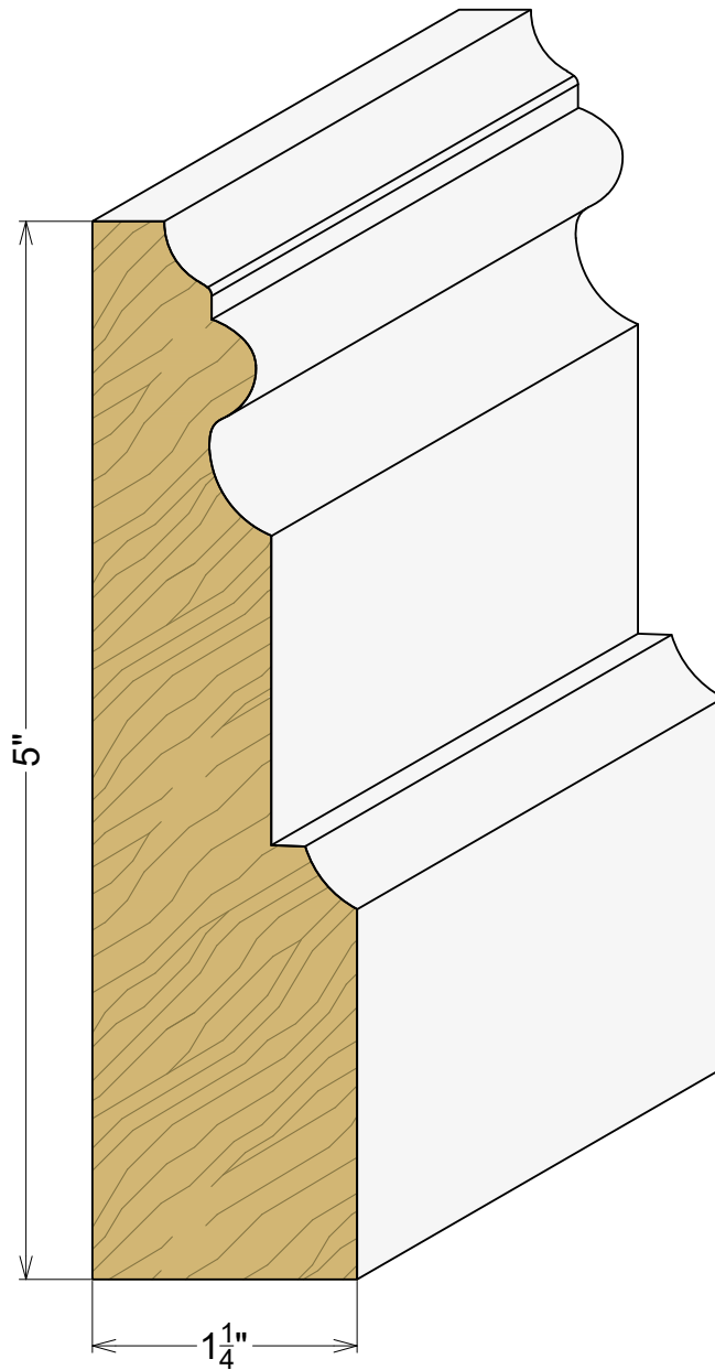
AP 2259 1-1/4" x 5"
