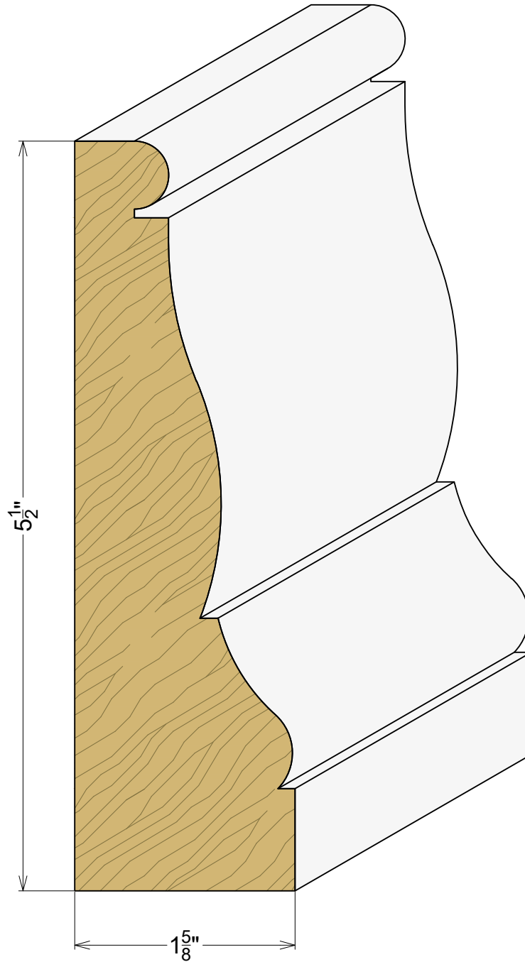
AP 2287 1-5/8" x 5-1/2"
