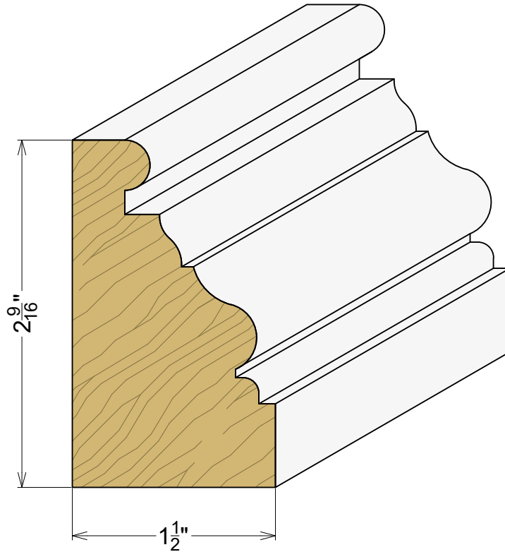
AP 2288 1-1/2" x 2-9/16"
