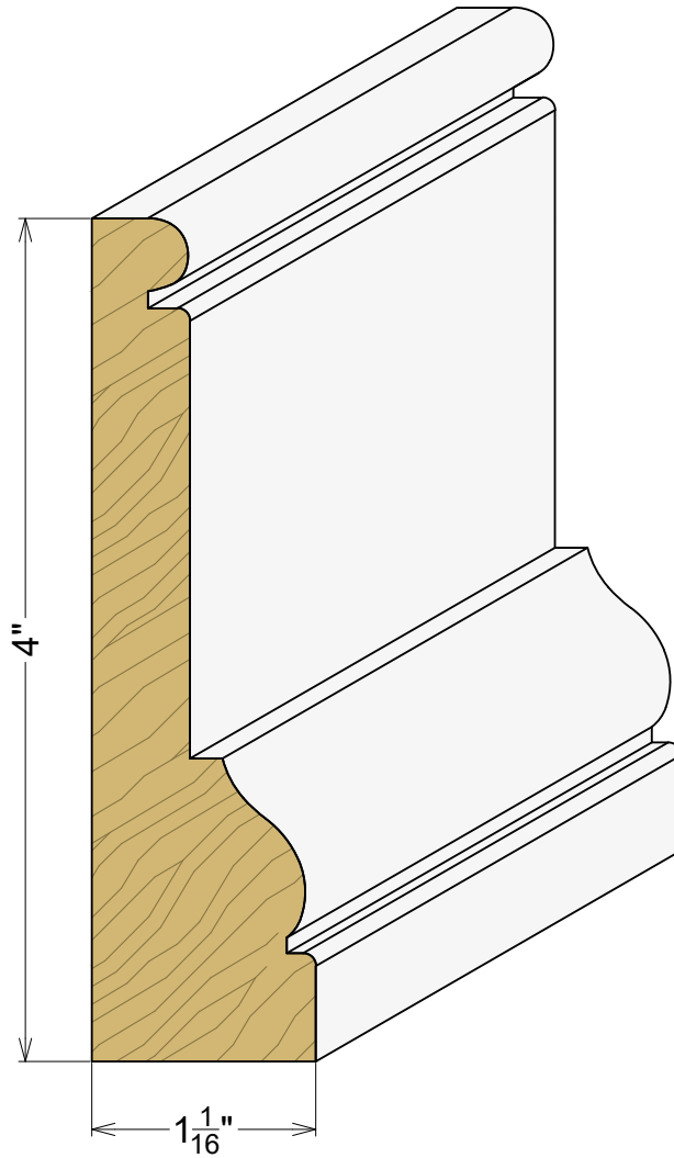
AP 2303 1-1/16" x 4"
