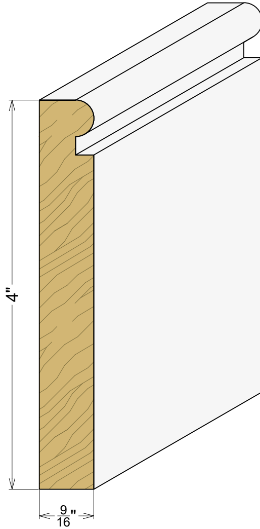
AP 2304 9/16" x 4"
