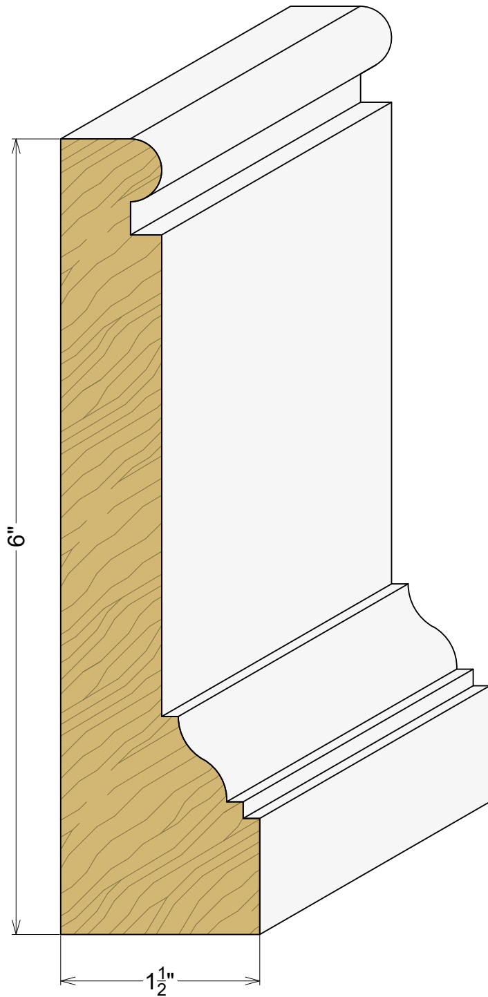
AP 2315 1-1/2" x 6"
