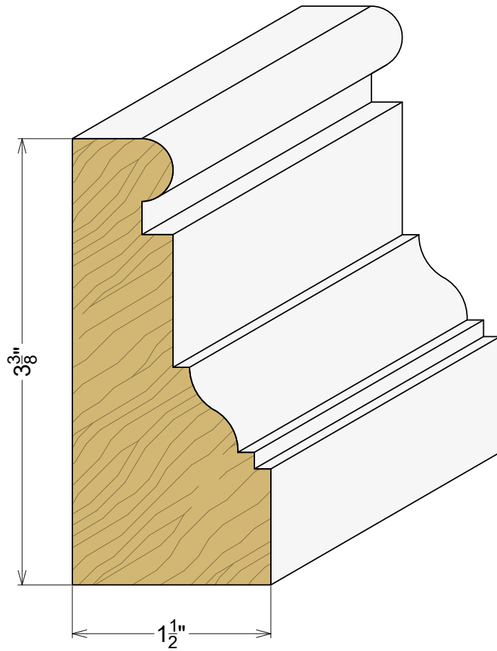
AP 2318 1-1/2" x 3-3/8"
