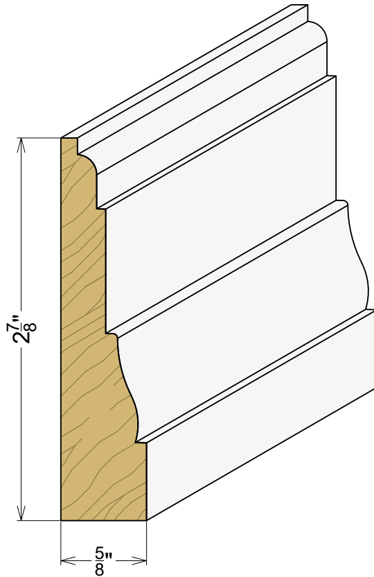
AP 2324 5/8" x 2-7/8"
