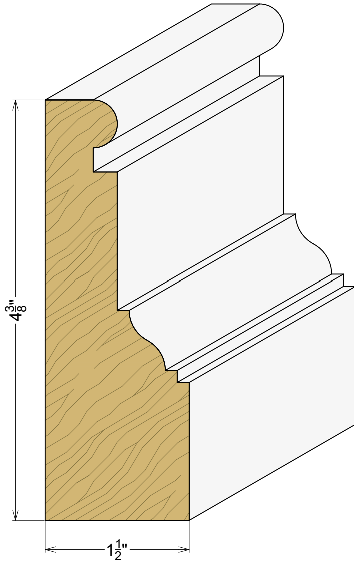
AP 2327 1-1/2" x 4-3/8"
