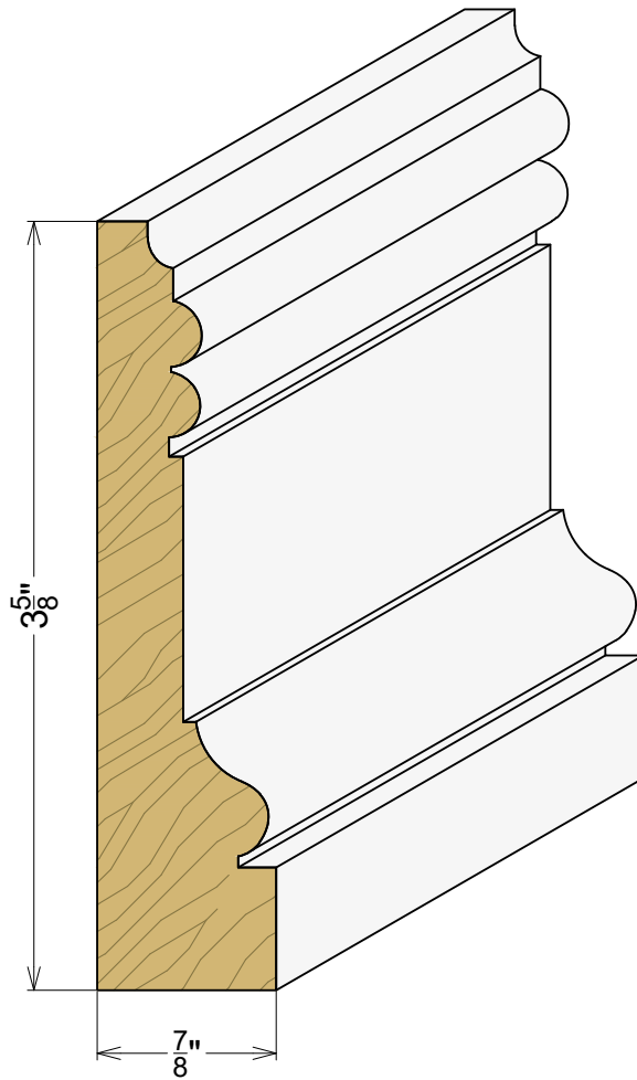
AP 2331 7/8" x 3-5/8"
