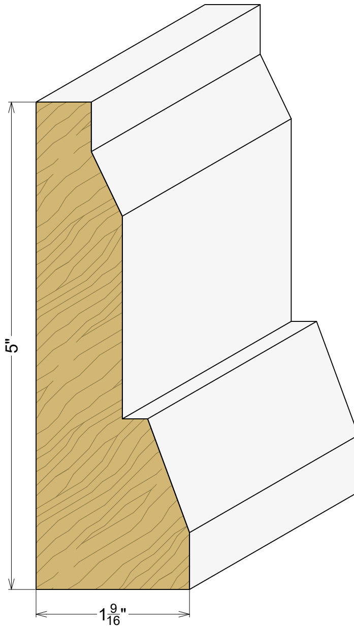
AP 2334 1-9/16" x 5" Plinth Block
