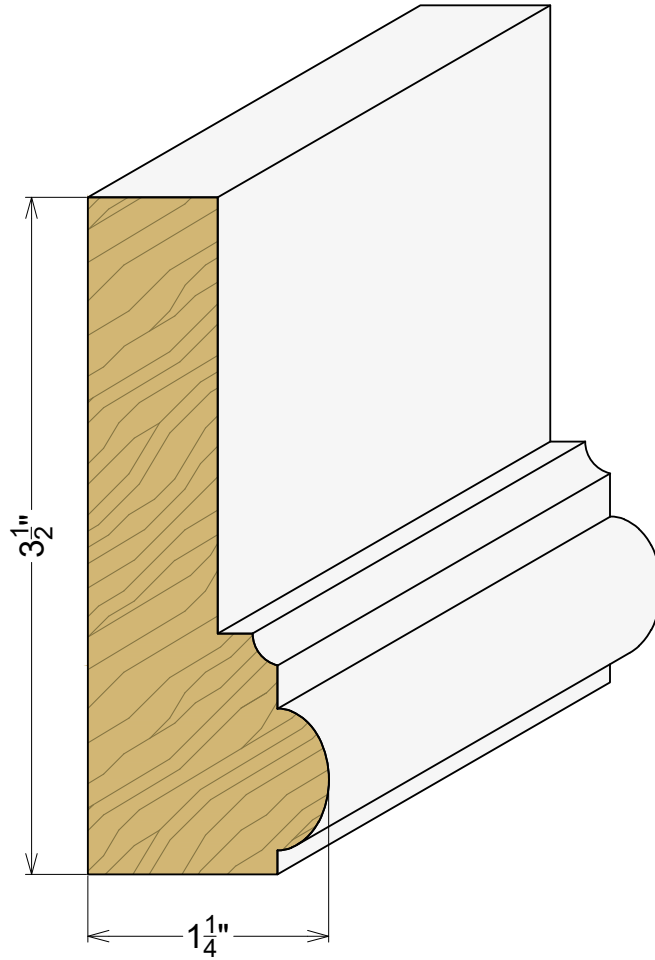
AP 2341 1-1/4" x 3-1/2"
