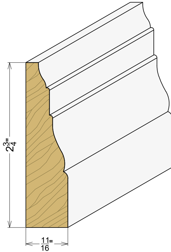
AP 2348 11/16" x 2-3/4"
