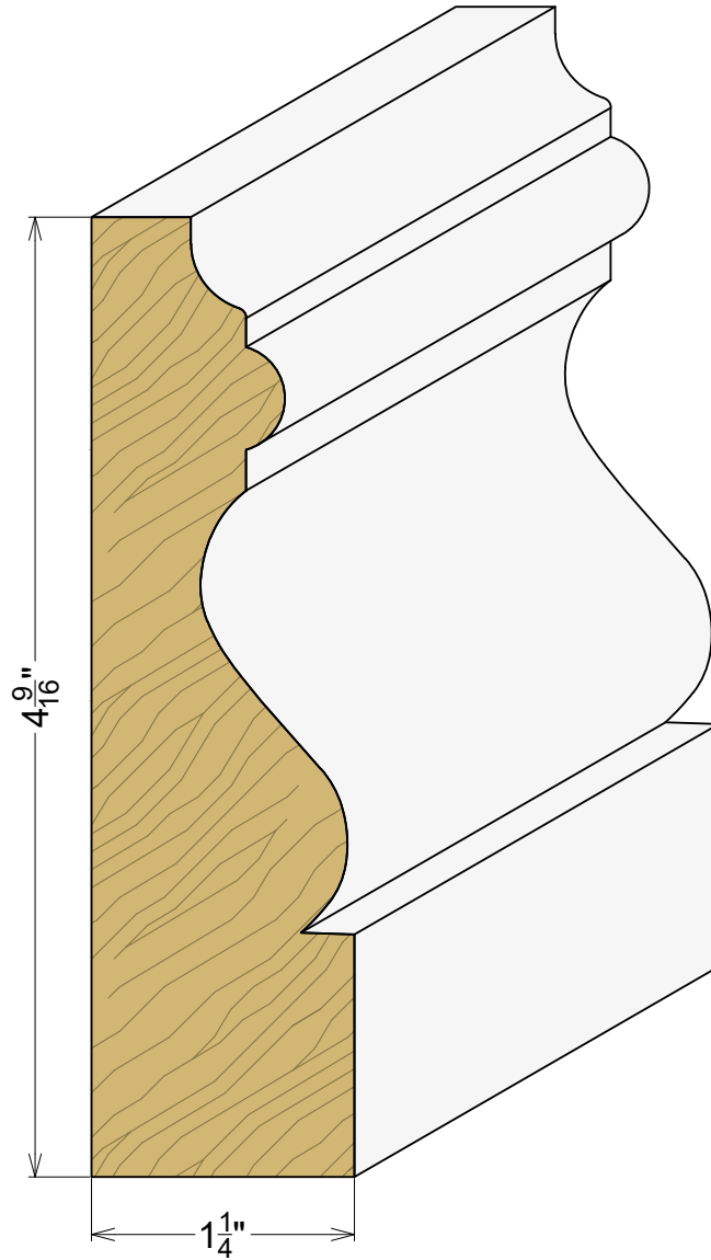
AP 2353 1-1/4" x 4-9/16"
