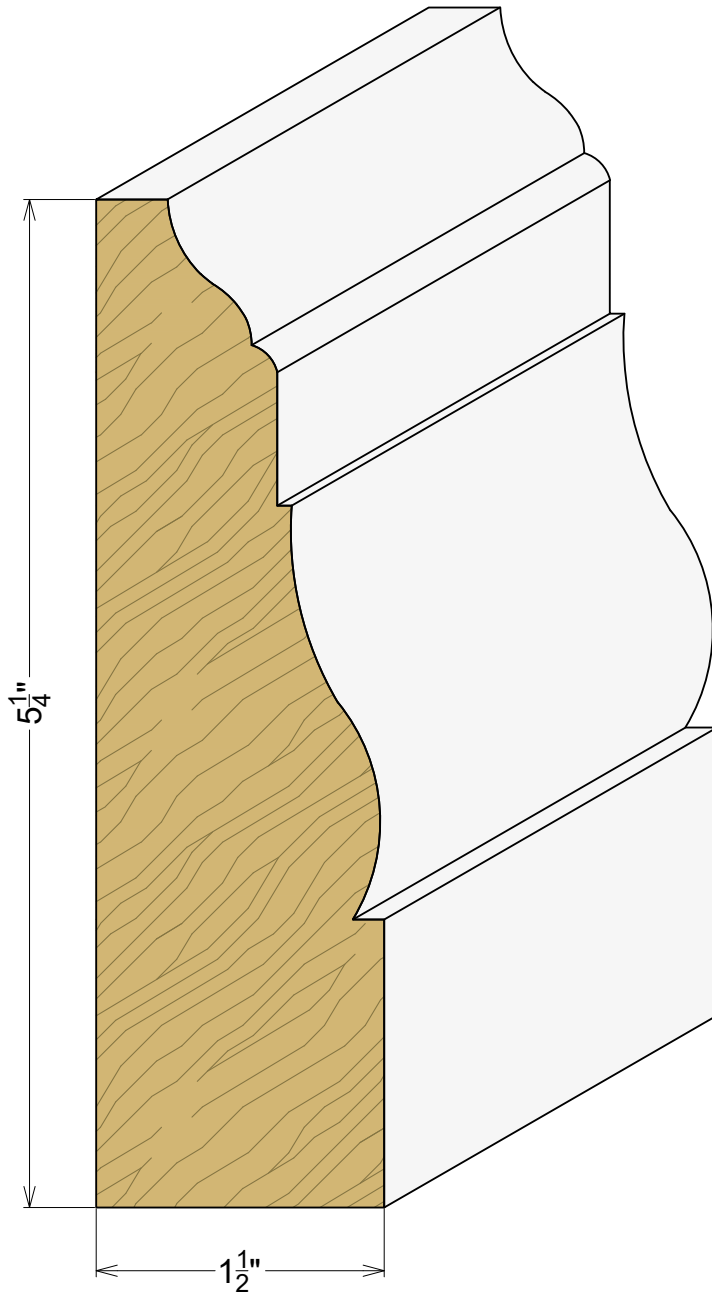
AP 2360 1-1/2" x 5-1/4"
