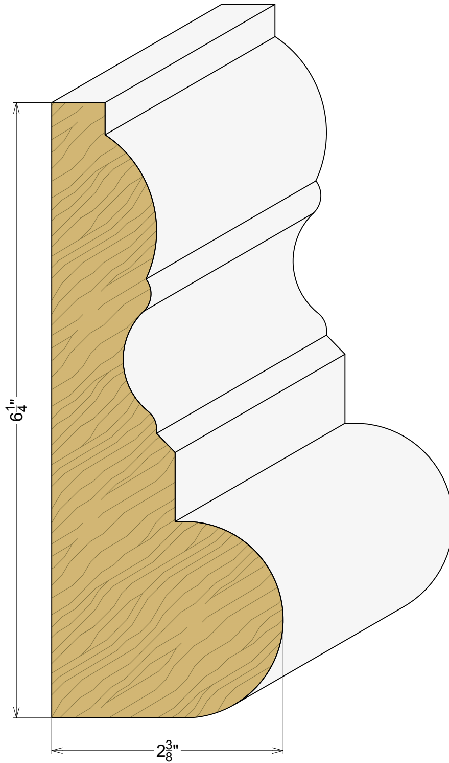
AP 2361 2-3/8" x 6-1/4" Plinth Block
