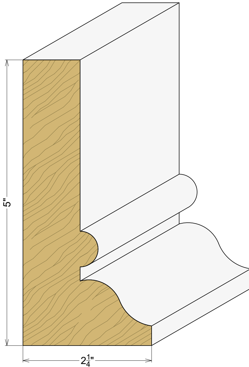
AP 2374 2-1/4" x 5"
