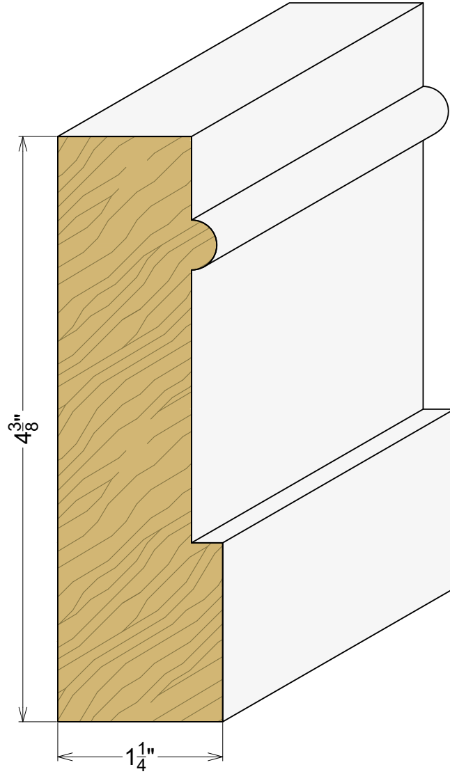
AP 2394 1-1/4" x 4-3/8"
