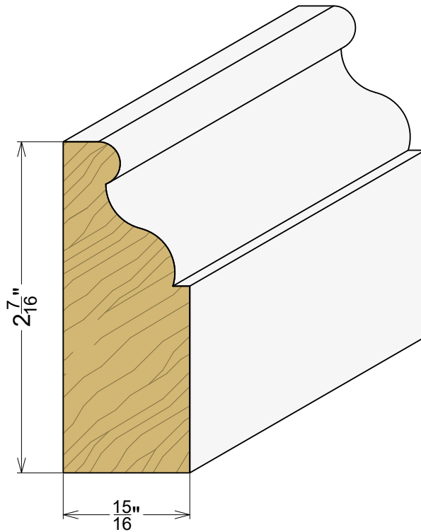
AP 2407 1 5/16" x 2 7/16"
