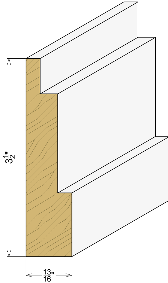
AP 2431 13/16" x 3-1/2"
