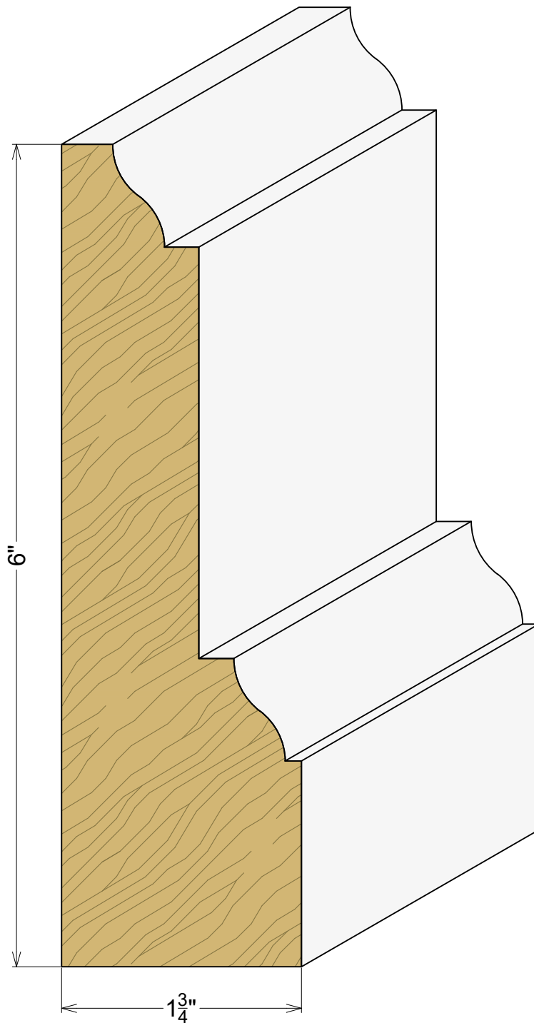
AP 2435 1-3/4" x 6"
