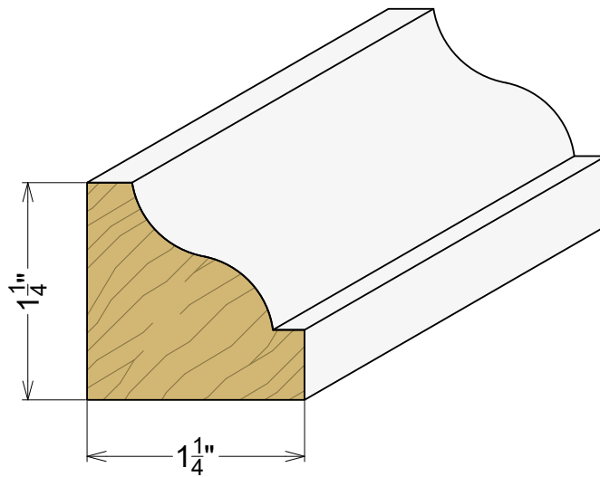
AP 2459 1-1/4" x 1-1/4"
