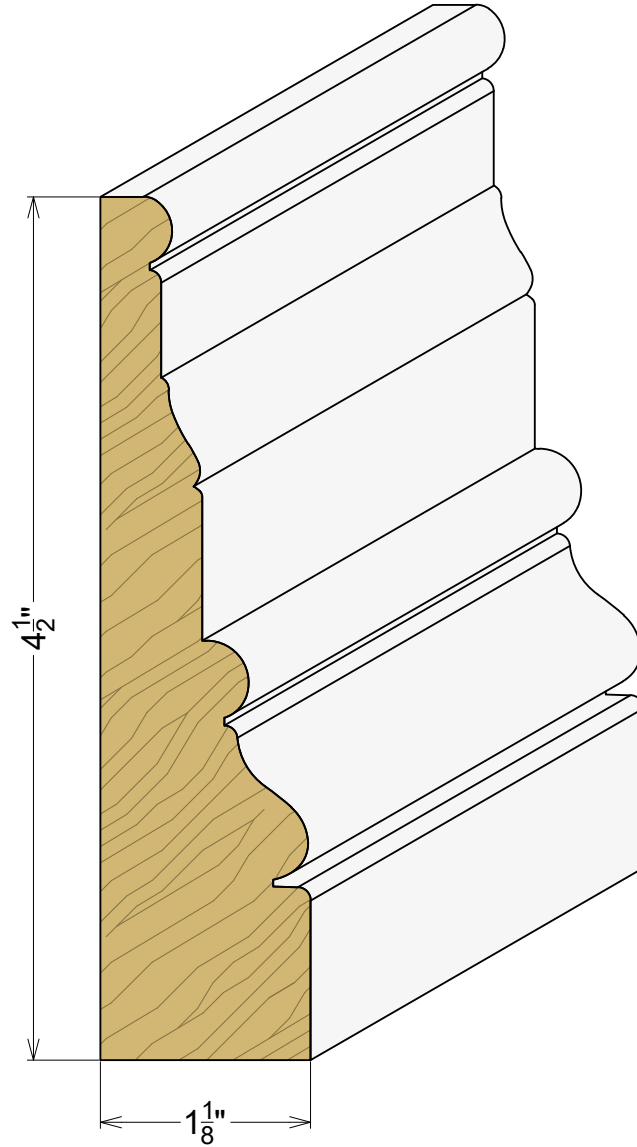
AP 2463 1-1/8" x 4-1/2"
