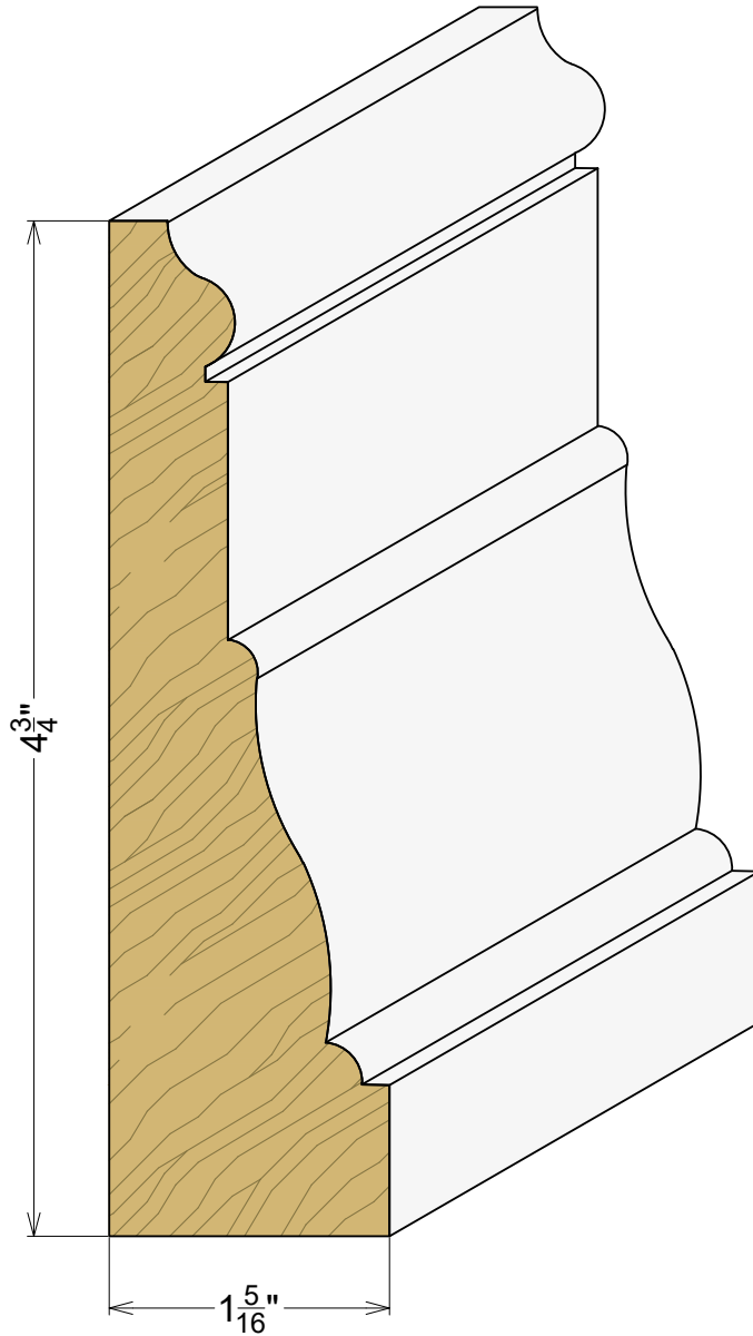
AP 2475 1-5/16" x 4-3/4"
