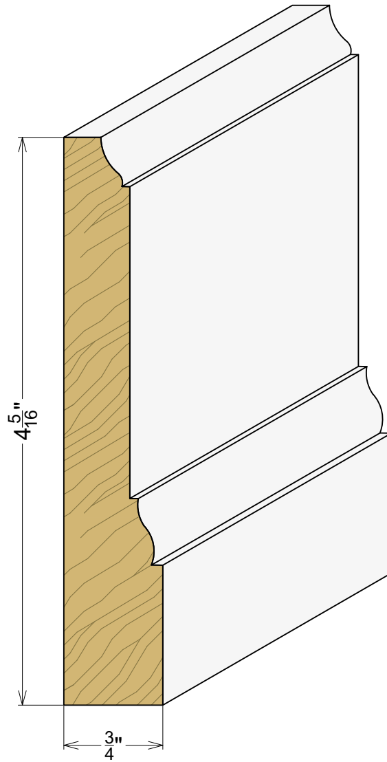
AP 2487 3/4" x 4-5/16"
