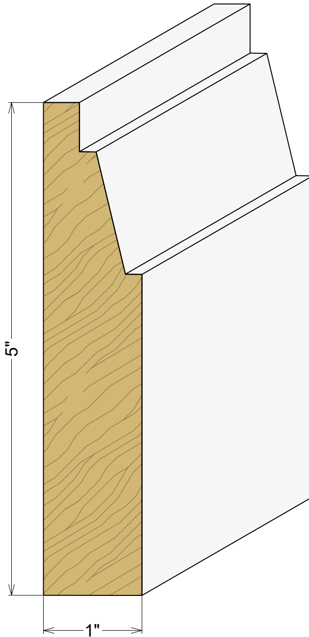
AP 2492 1" x 5"
