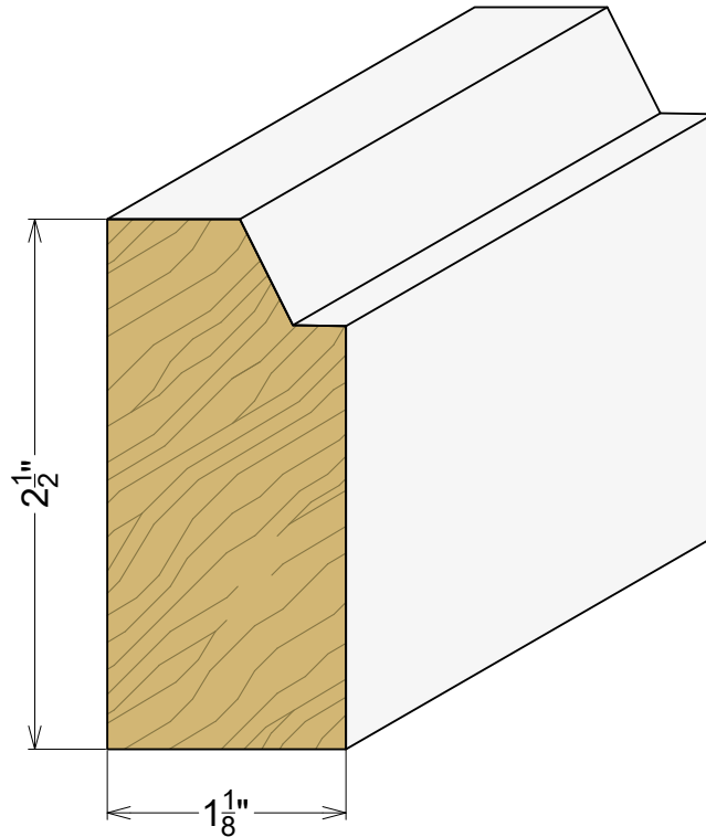
AP 2496 1-1/8" x up to 9-1/4"
