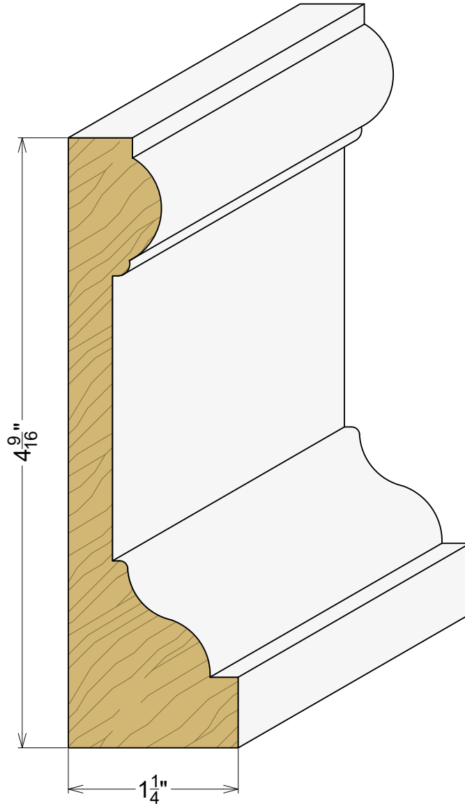
AP 2512 1-1/4" x 4-9/16"
