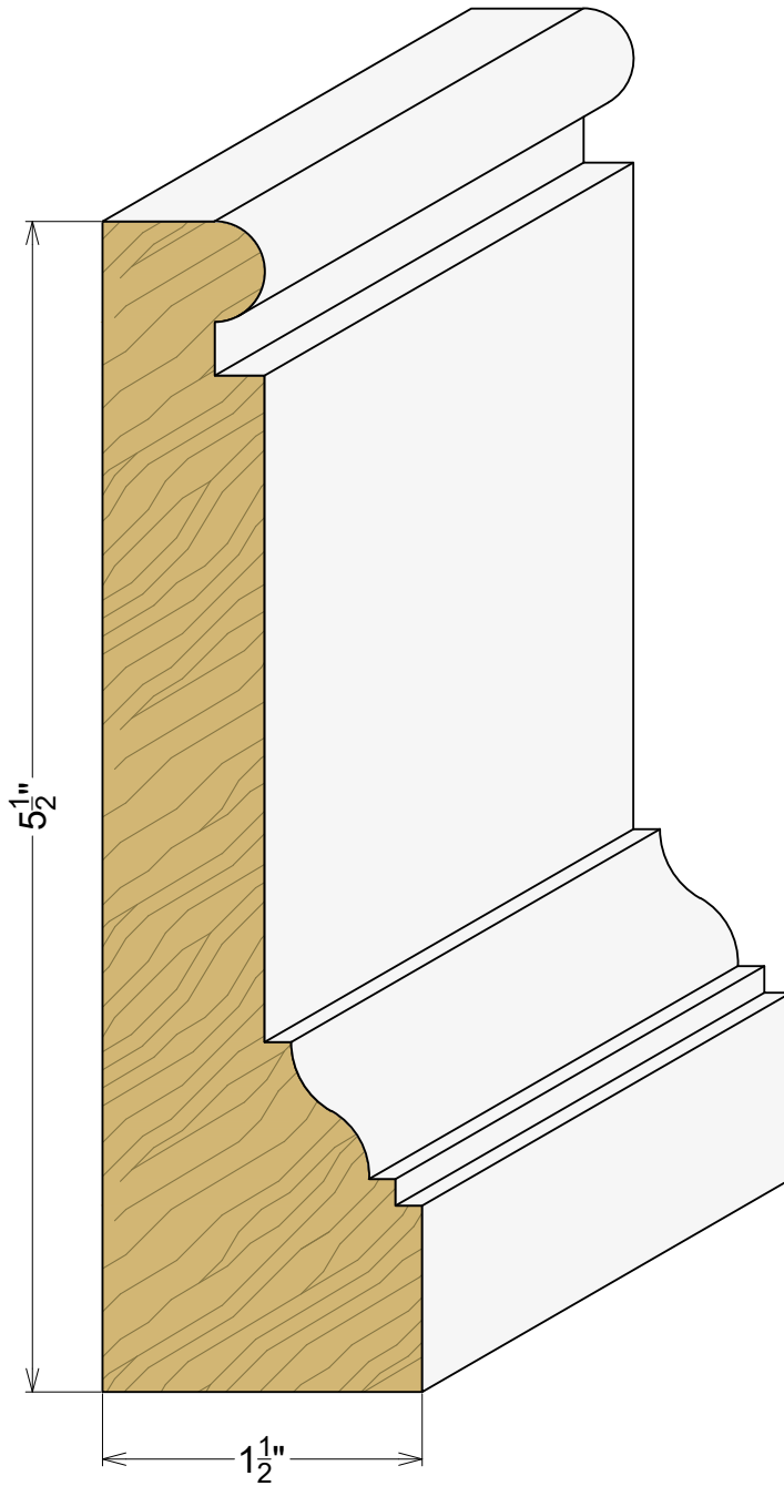
AP 2518 1-1/2" x 5-1/2"
