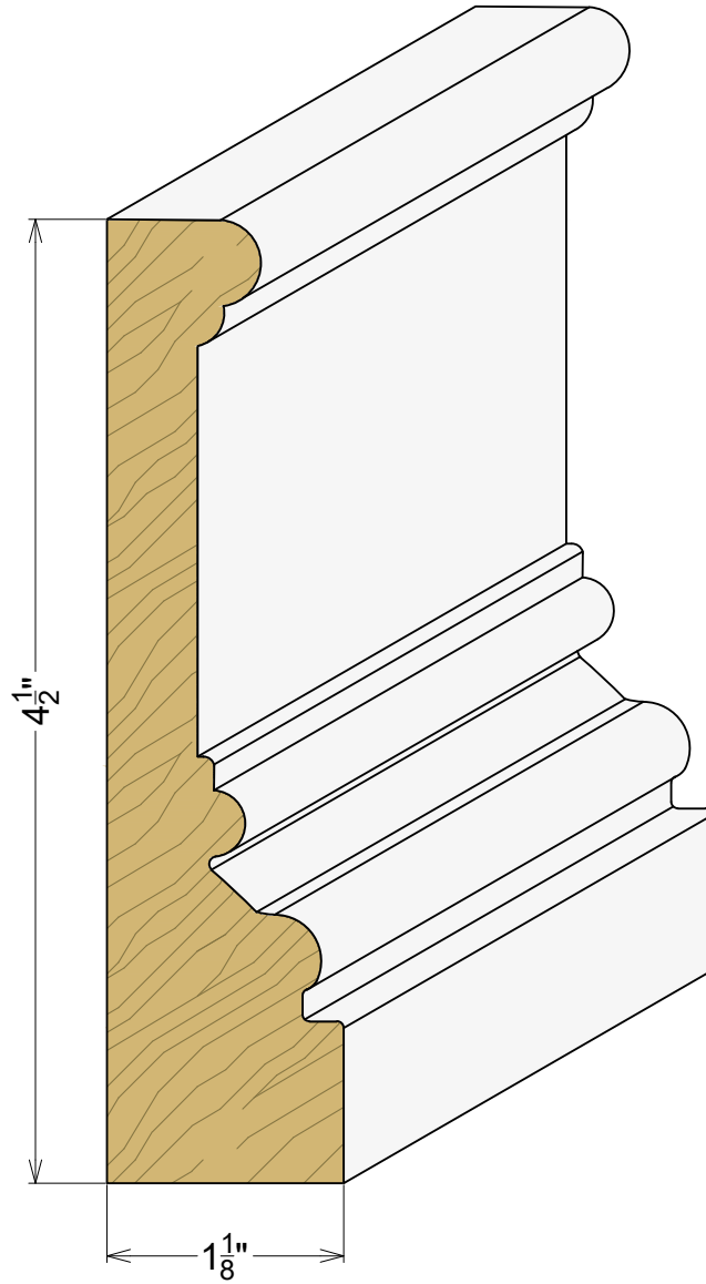
AP 2534 1-1/8" x 4-1/2"
