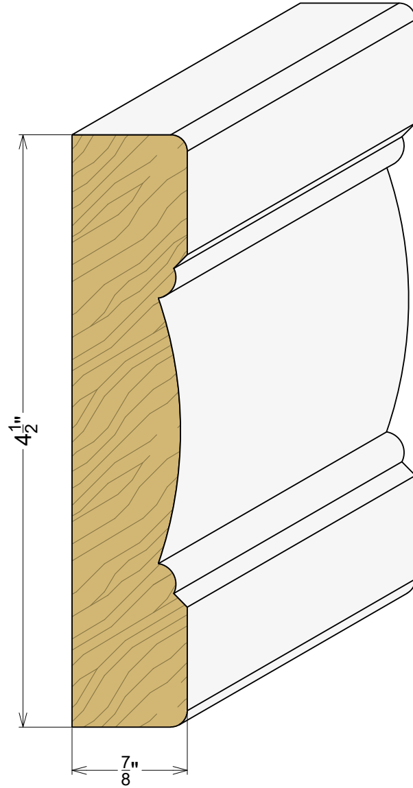
AP 2538 7/8" x 4-1/2"
