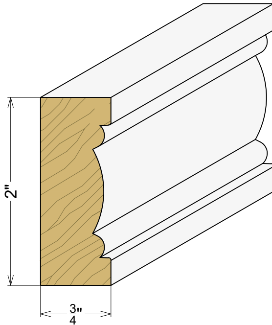
AP 2551 3/4" x 2"
