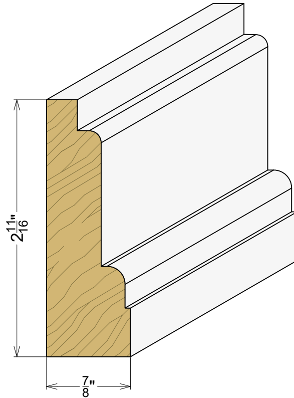
AP 2552 7/8" x 2-11/16"
