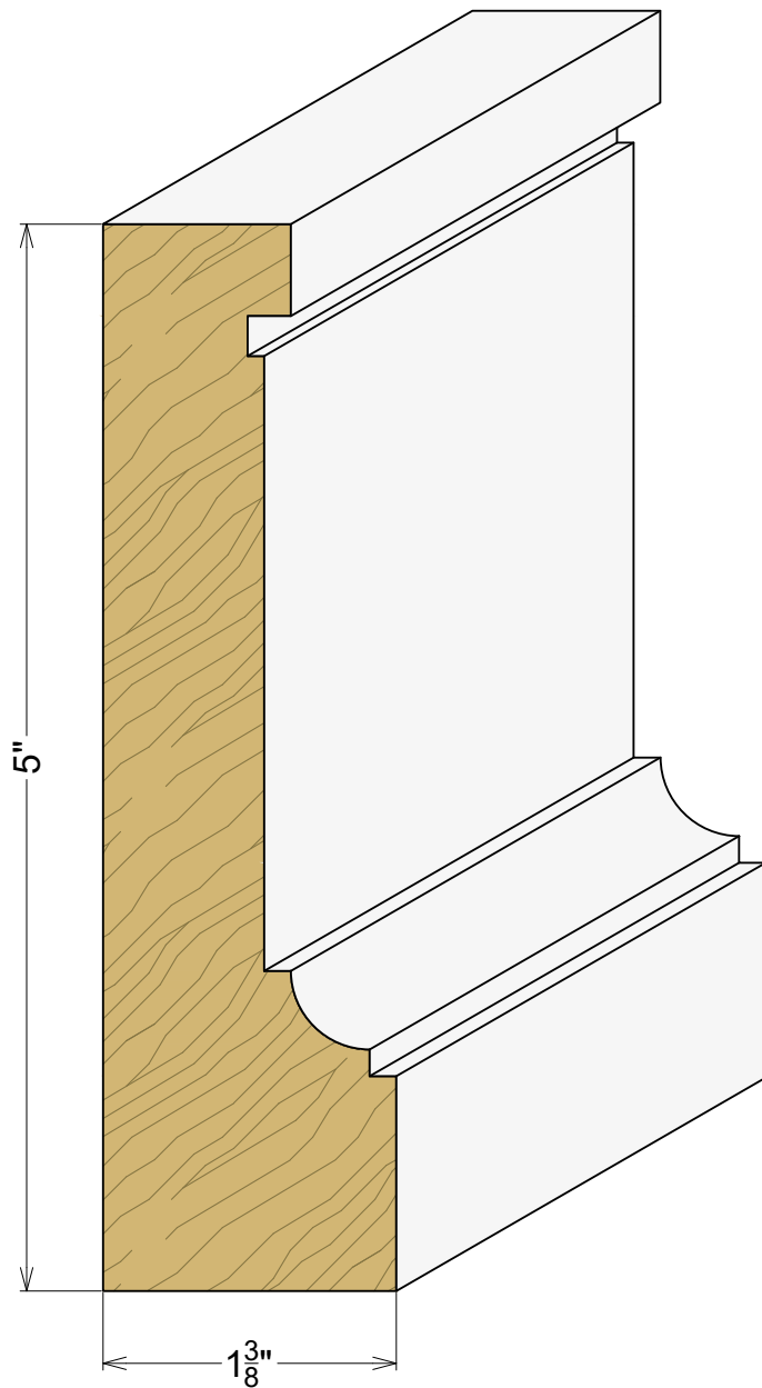
AP 2555 1-3/8" x 5"
