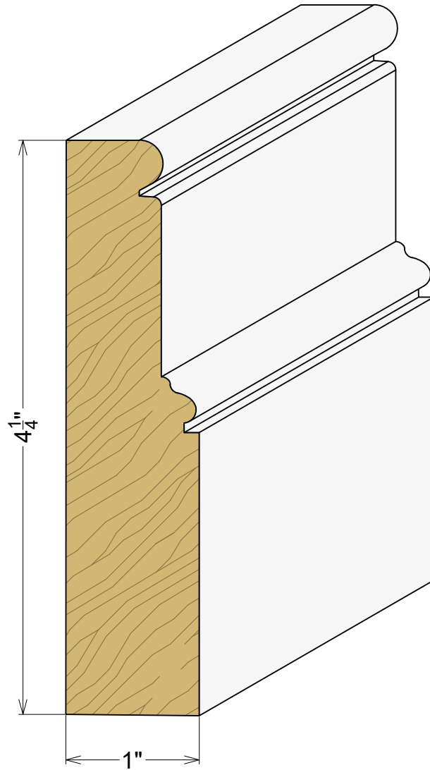
AP 2561 1" x 4-1/4"
