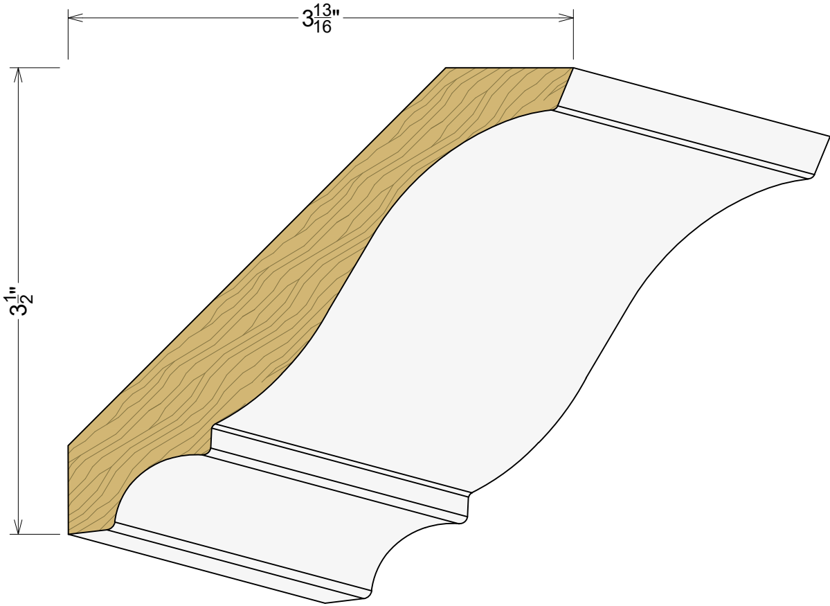
AP 3701 3/4"x 5 3/16"
