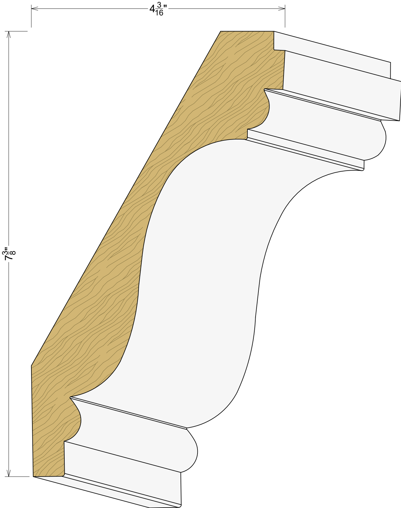
AP 3704 1 3/8"x 8 3/8"
