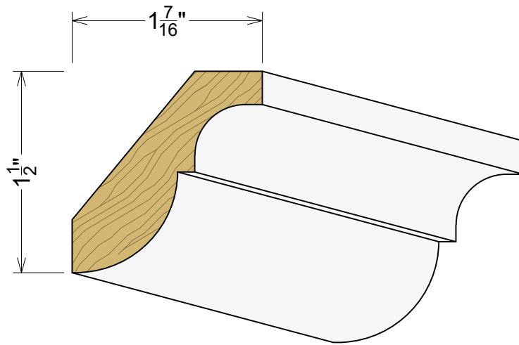
AP 3705 17/32"x 2 1/16"
