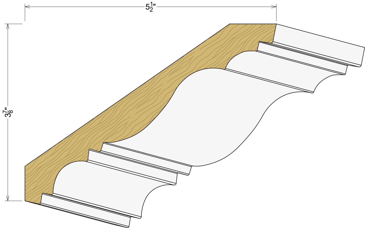
AP 3717 7/8" x 6 3/4"
