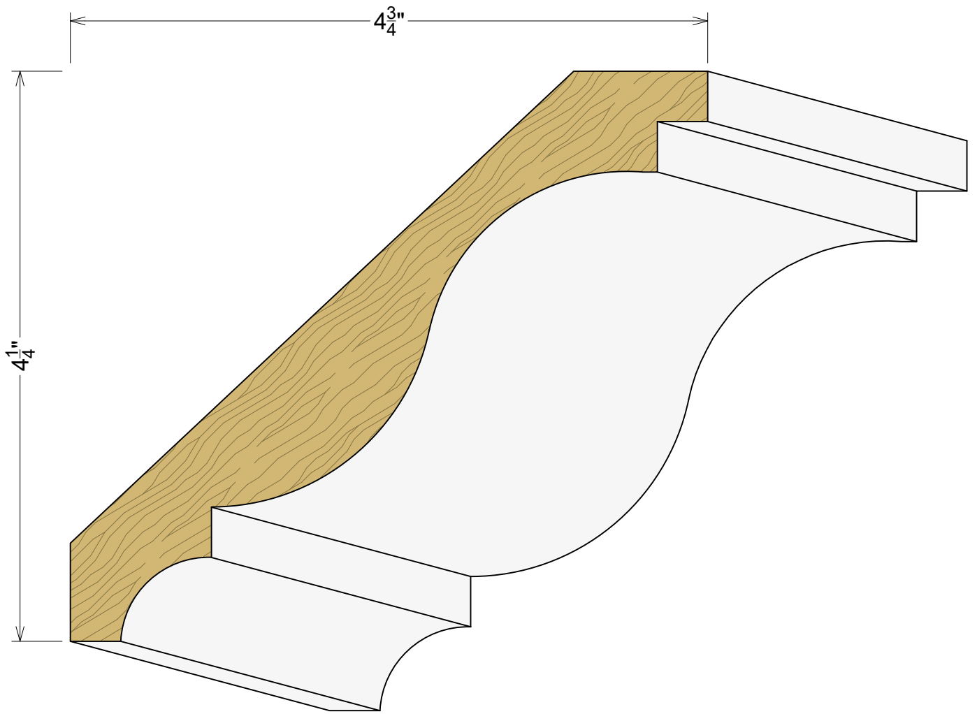
AP 3739 1"x 6 3/8"
