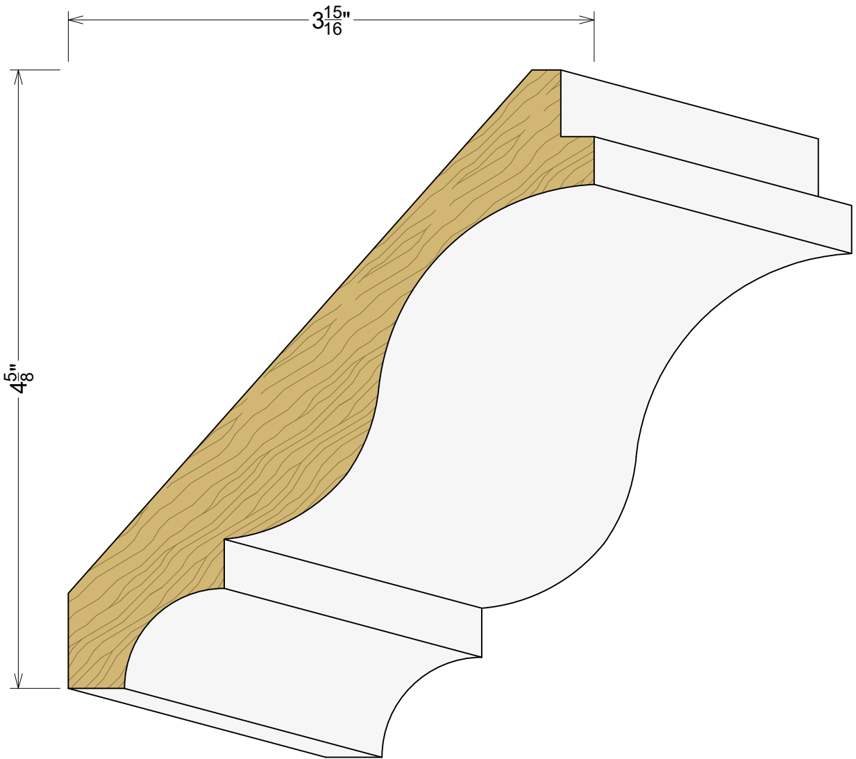
AP 3744 1"x 5 15/16"
