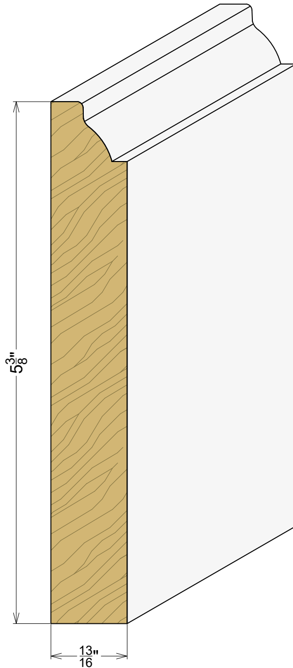
AP 4227 13/16" x 5-3/8"
