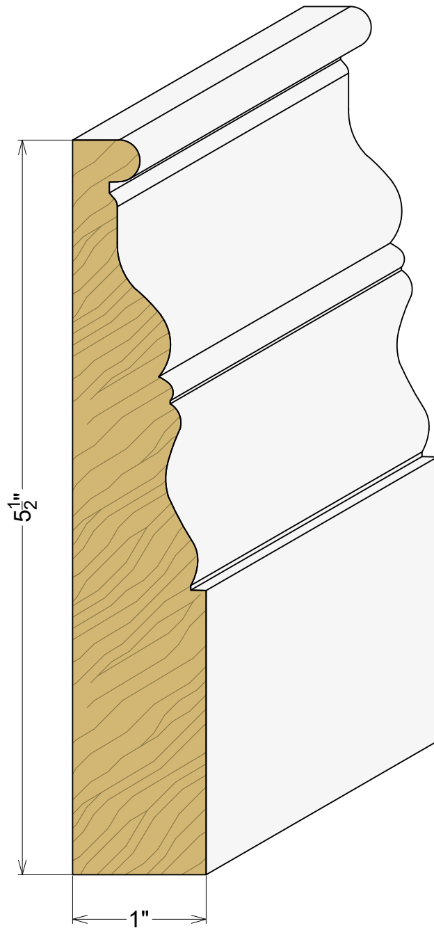
AP 4251 1" x 5-1/2"
