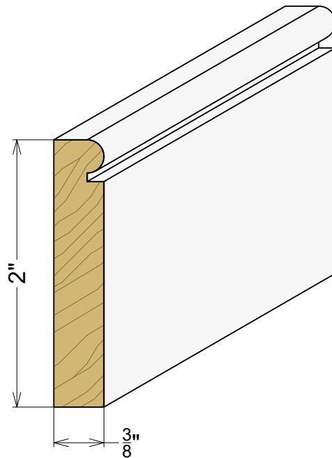
AP 4259 3/8" x 2"
