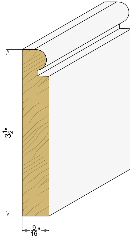
AP 4302 9/16" x 3-1/2"
