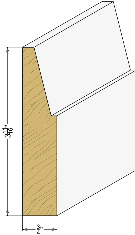
AP 4412 3/4" x up to 9-1/4"
